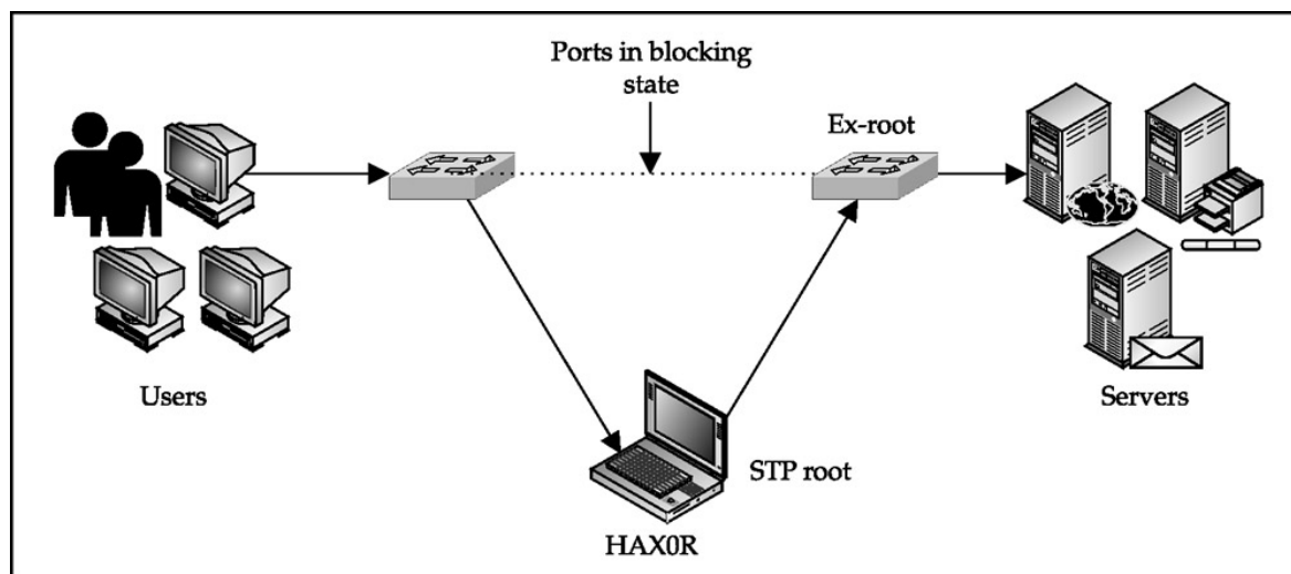
Figura 9 – Spanning Tree Protocol Attack
